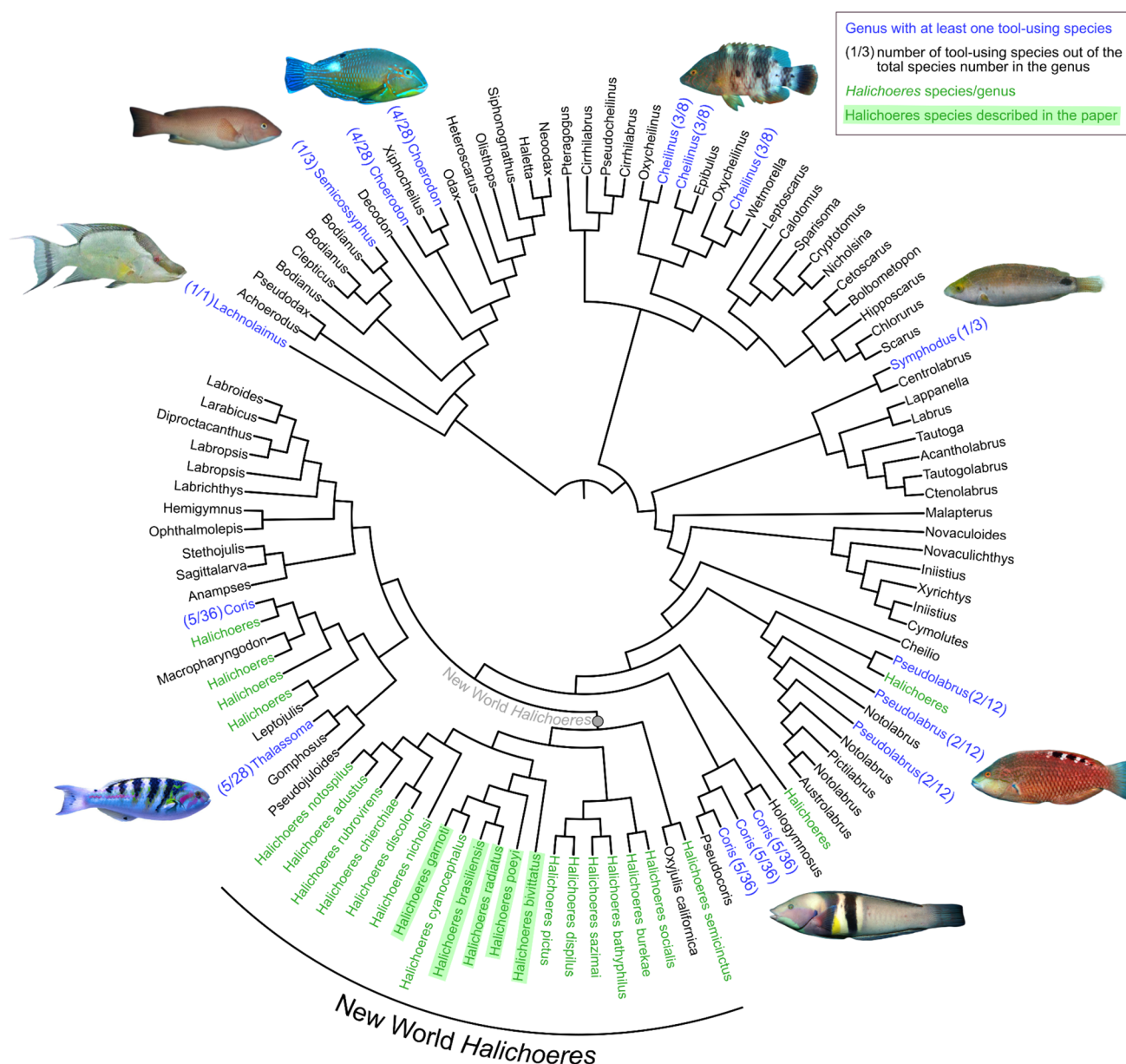
Fig. 1 Tool-using genera within the Labridae family. Labridae phylogeny has been simplified to the genus level except for the New World Halichoeres , for which species have been plotted. Some genera are polyphyletic and appear multiple times in the tree, such as Choerodon , Cheilinus , or Coris . Blue indicates a genus in which at least
